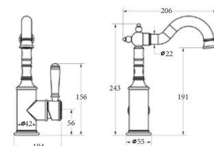
HYB868-202 HYB868-202A-BG HYB868-202A-BN HYB868-202A-MB
