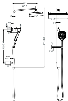
PHC636-201 PHC636-201BN PHC636-201MB
